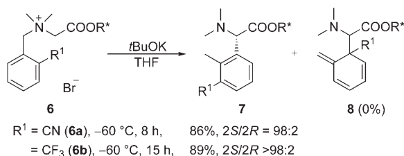
Scheme 2. Asymmetric Sommelet–Hauser rearrangement of ortho -substituted N -benzylic ammonium salt 6 . \text{R}^* = (-) -8-phenylmenthyl.
