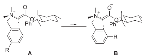
Scheme 3. Proposed intermediates in the asymmetric Sommelet–Hauser rearrangement of meta -substituted N -benzylic ammonium salt 9 . Intermediate A leads to compound 10 (2,4-disubstituted), whereas intermediate B leads to compound 11 (2,6-disubstituted).
