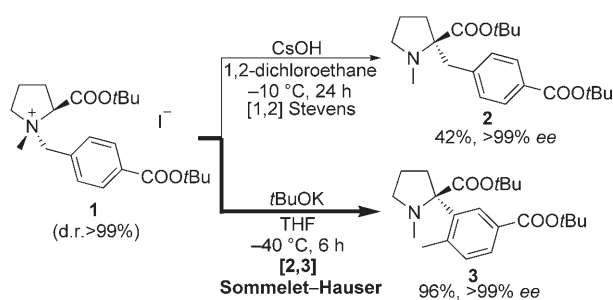
Scheme 1. The [1,2] Stevens versus Sommelet–Hauser rearrangement.
